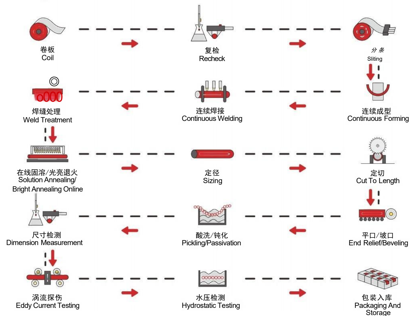
连续成型焊管生产工艺流程图 Process Flow Chart for Continuous Forming Welded Pipe Production
